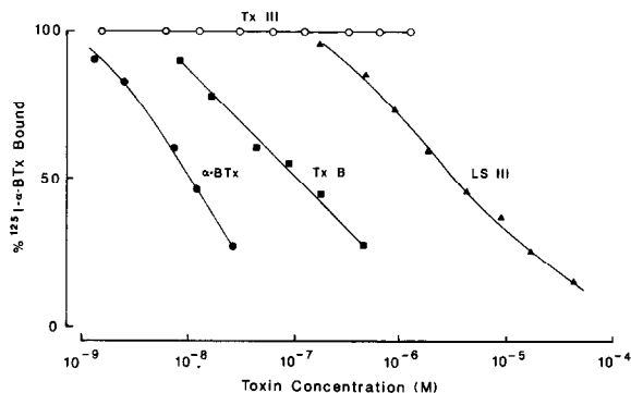
Fig.1. Binding of ^{125} I-labeled \alpha -bungarotoxin ( \alpha -BTx) to monoclonal antibody MaB-2311 in the presence of varying amounts of unlabeled \alpha -bungarotoxin ( \alpha -BTx), toxin B (Tx B), toxin III (Tx III) or Ls III. In these experiments, 6 nM monoclonal antibody was incubated with 6.5 nM ^{125} I-labeled \alpha -bungarotoxin and varying amounts of long neurotoxins.
